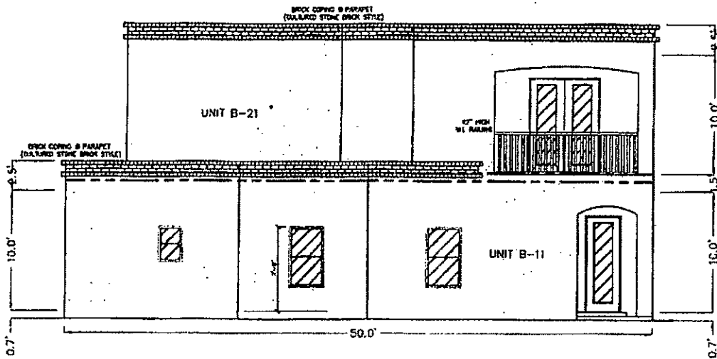
REAR ELEVATION
