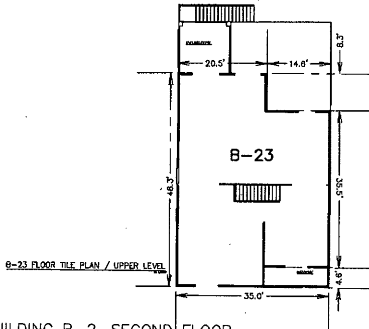
BUILDING B-2, SECOND FLOOR
