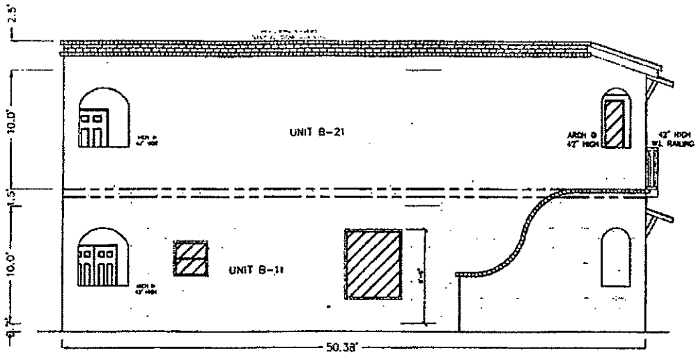
LEFT ELEVATION
