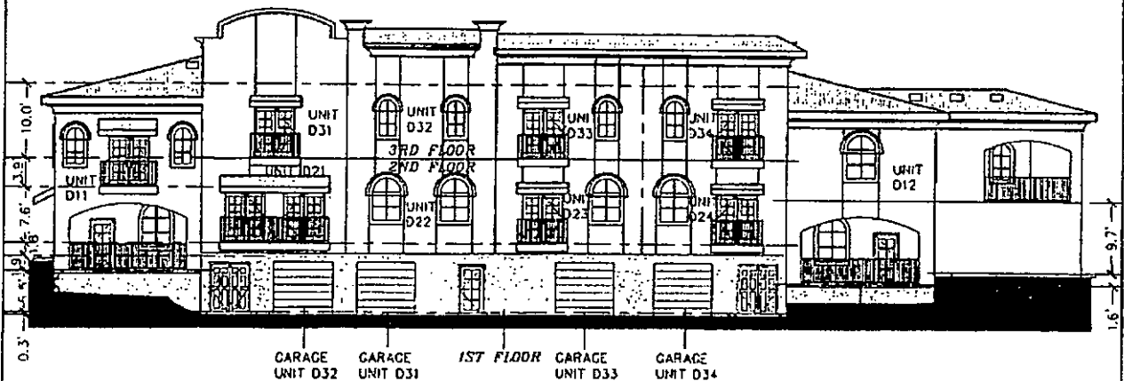
BUILDING D WEST ELEVATION
