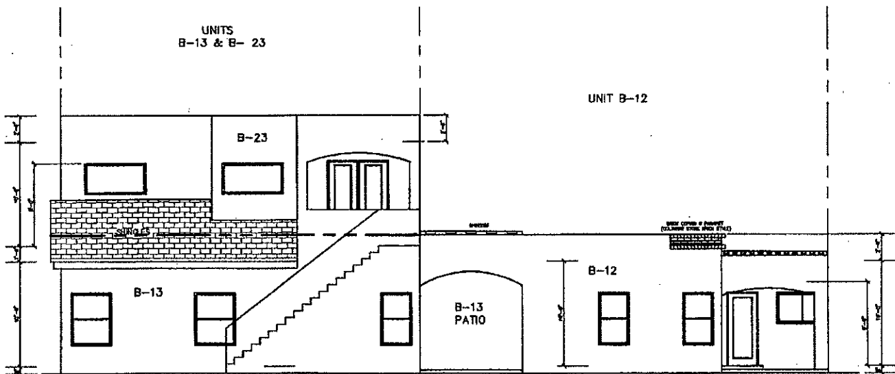
BUILDING B SOUTH ELEVATION
