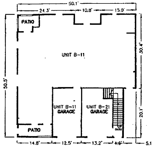
BUILDING B-1 FIRST FLOOR
