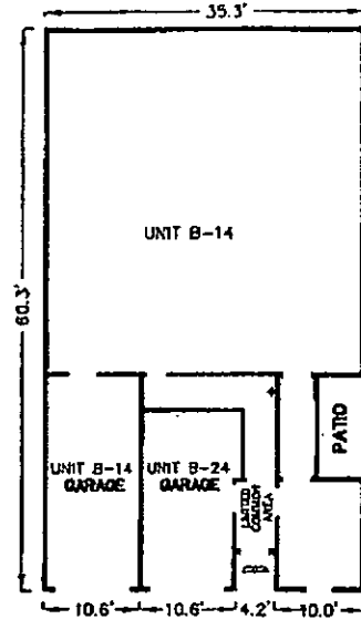
BUILDING B-4 FIRST FLOOR
