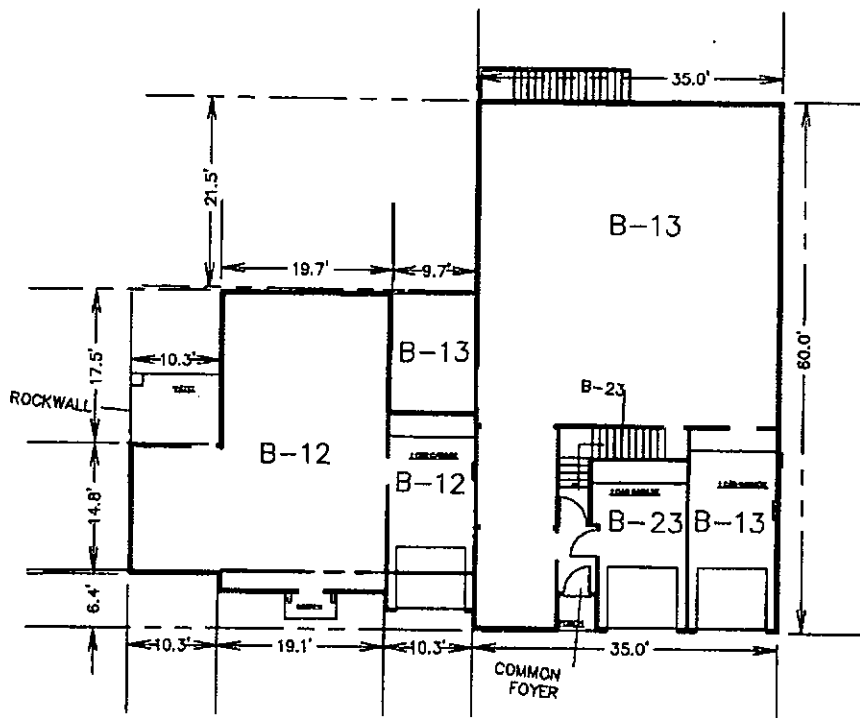
BUILDING B-2, FIRST FLOOR
