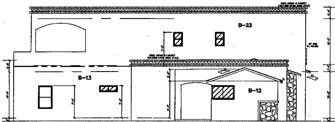
LEFT ELEVATION
