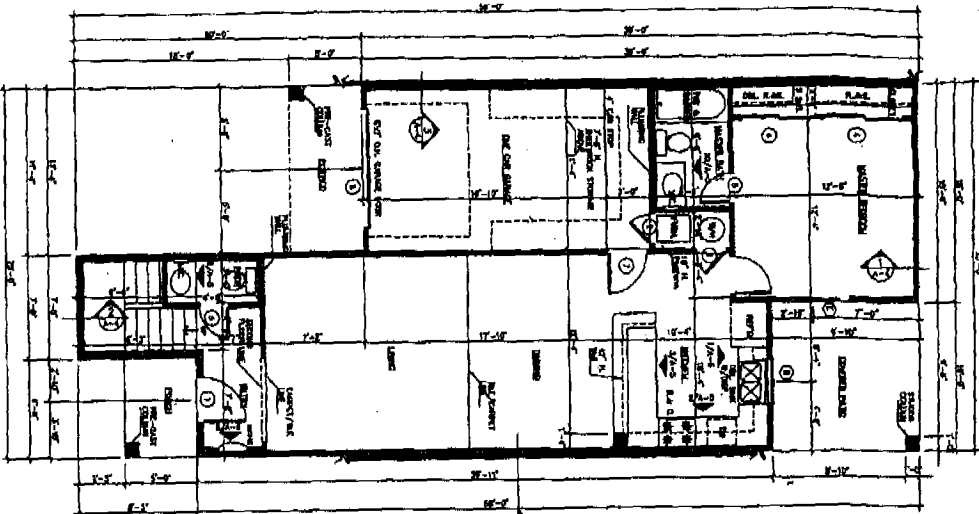
FIRST FLOOR PLAN - 3 BEDROOM UNIT SCALE 1/8" = 1'-0"
