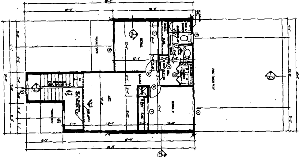
SECOND FLOOR PLAN - 3 BEDROOM UNIT SCALE 1/8" = 1'-0"
